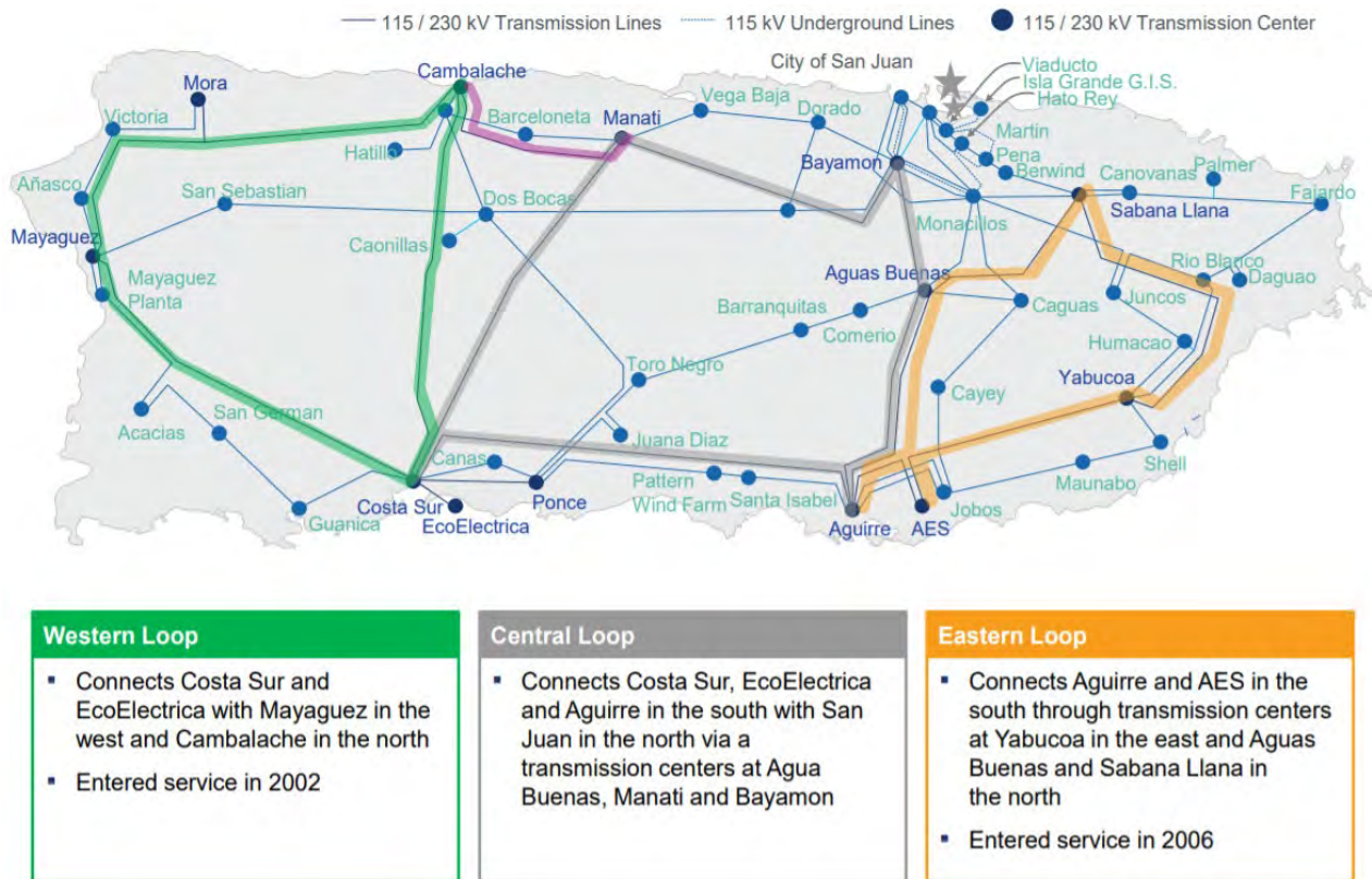
Figure 58. Map of PREPA transmission and distribution lines. Source: 2019 Fiscal Plan for the
